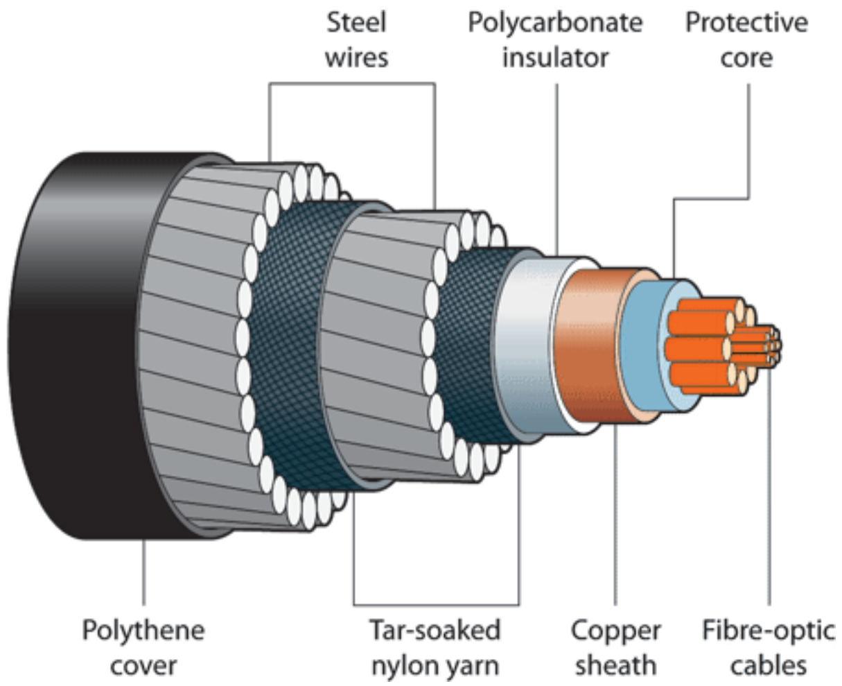
Cross section of undersea internet cables
